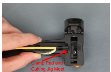
Step 9: Slide the cutting jig in the holder slot of the cleaver until the end of the cutting jig meets the clamp pad. Cleave fiber.
